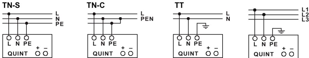
Figure 6 Network types
