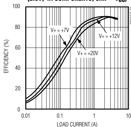
EFFICIENCY vs. LOAD CURRENT (2.5V, 4A COMPONENTS, \overline{SKIP} = V_{CC} )
