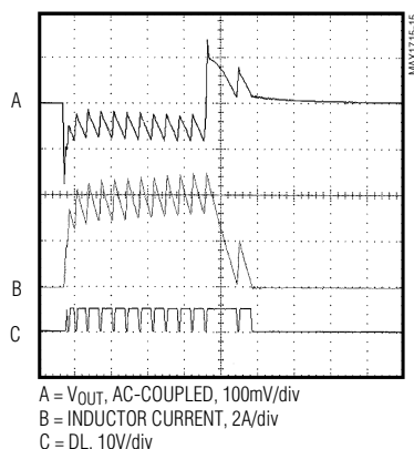
OUTPUT OVERLOAD WAVEFORM (2.5V, 4A COMPONENTS, SKIP = GND)
