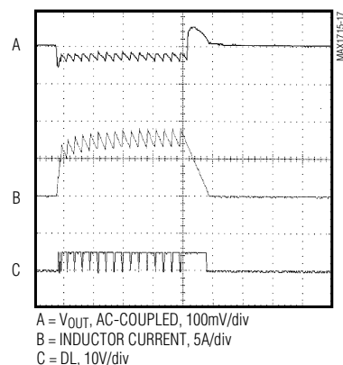
LOAD-TRANSIENT RESPONSE (1.3V, 8A COMPONENTS, SKIP = GND)
