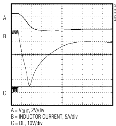
SHUTDOWN WAVEFORM (2.5V, 4A COMPONENTS, SKIP = GND)
