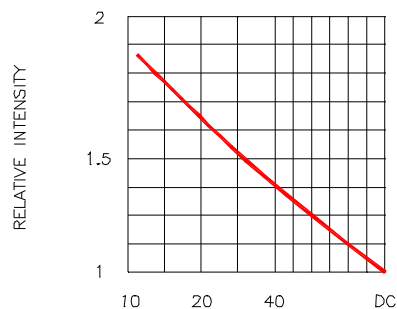
Fig.4 LUMINOUS INTENSITY VS. DUTY CYCLE (AVERAGE IF=10mA)
