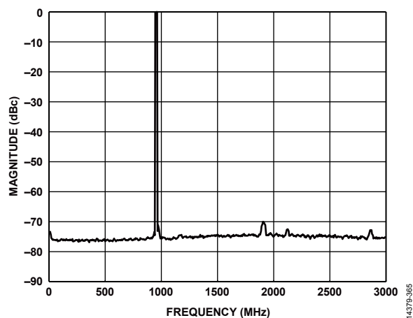
Figure 121. Four Carriers at 950 MHz Output (Shuffle On)
