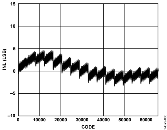
Figure 59. INL, I_{OUTFS} = 30 mA
