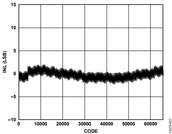
Figure 60. INL, I_{OUTFS} = 40 mA
