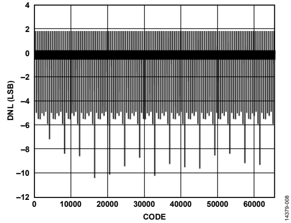
Figure 61. DNL, I_{OUTFS} = 20 mA
