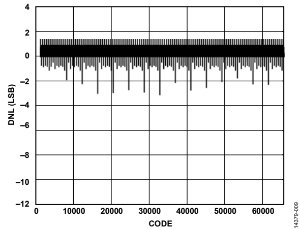
Figure 62. DNL, I_{OUTFS} = 30 mA
