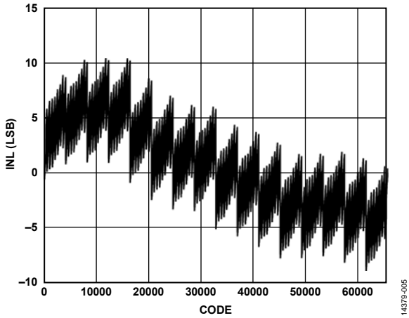
Figure 58. INL, I_{OUTFS} = 20 mA
