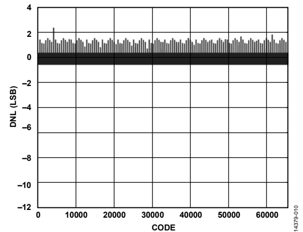
Figure 63. DNL, I_{OUTFS} = 40 mA
