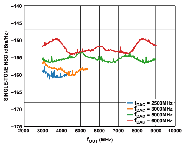
Figure 30. Single-Tone NSD Measured at 70 MHz vs. f_{OUT}
