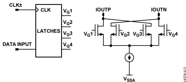
Figure 180. Quad-Switch Architecture
