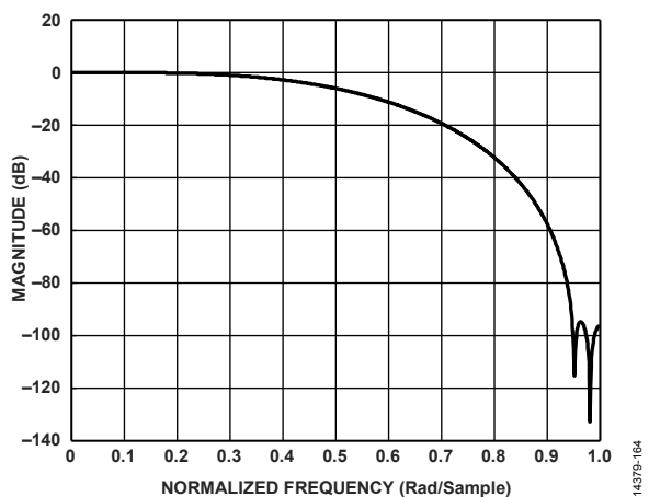
Figure 170. Fourth 2× Half-Band 11.25% Filter Response
