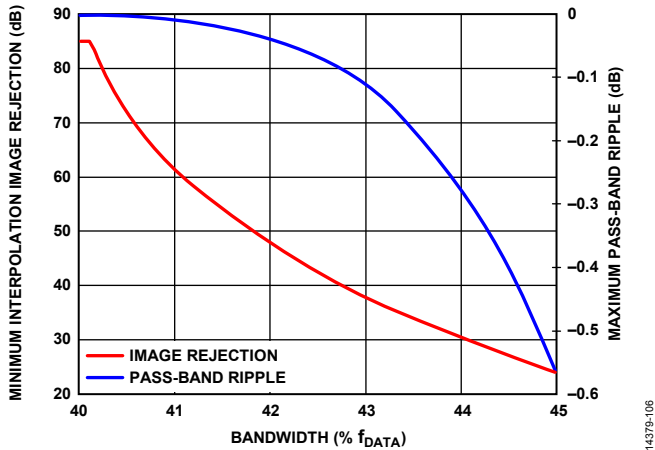
Figure 163. Interpolation Filter Performance Beyond Specified Bandwidth for the 80% Filters
