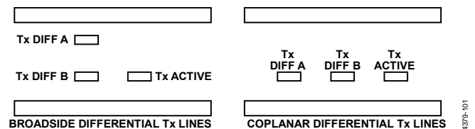
Figure 177. Broadside vs. Coplanar Differential Stripline Routing Techniques
