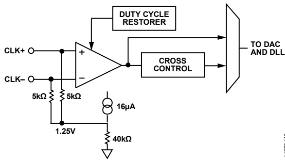
Figure 185. Clock Input
