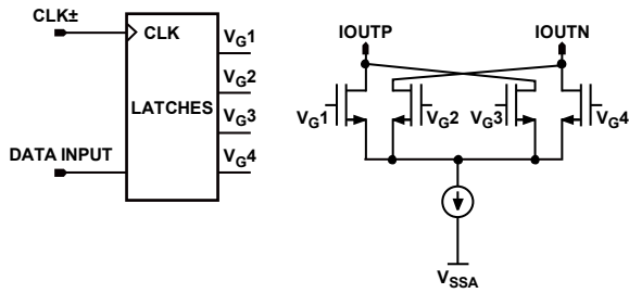
Figure 180. Quad-Switch Architecture
