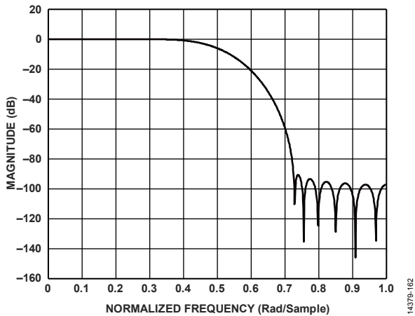
Figure 168. Second 2× Half-Band 45% Filter Response
