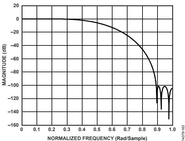
Figure 169. Third 2× Half-Band 22.5% Filter Response
