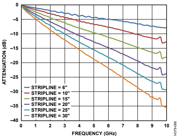
Figure 148. Insertion Loss of 50 Ohm Striplines on FR4
