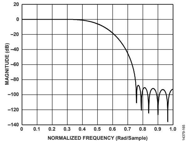
Figure 171. FIR85 2× Half-Band 45% Filter Response
