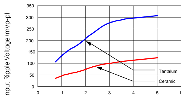
Figure 27. Input ripple voltage for various output with 2x47 μF tantalum capacitors and with 2x22 μF ceramic capacitors at the input (80% of I_{O,max} ).
