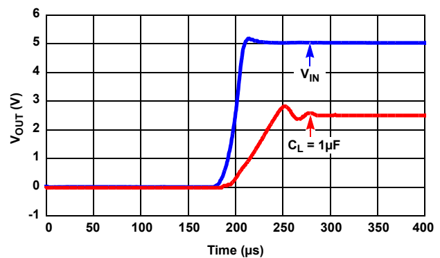
Figure 18. Turn-On Time with 1µF
