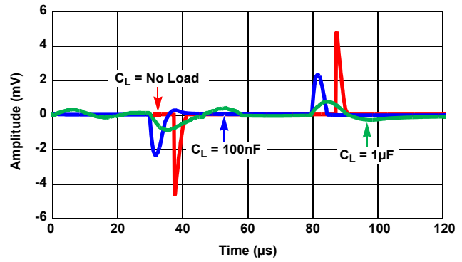
Figure 15. Load Transient ( \Delta I_{LOAD} = \pm 1mA )
