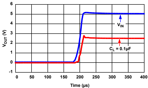
Figure 17. Turn-On Time with 0.1µF
