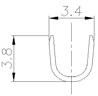
SEC. B-B
