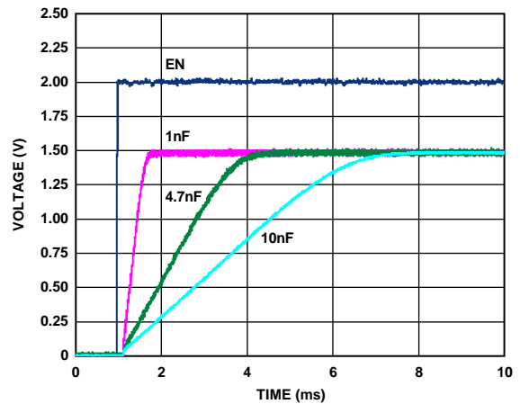
Figure 26. V OUT Ramp-Up with External Soft Start Capacitor
