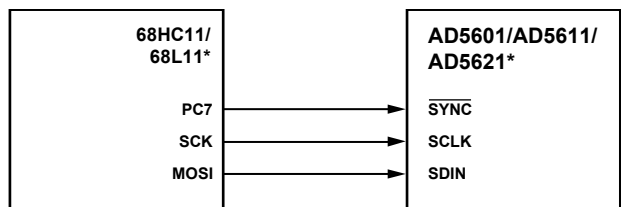
Figure 47. AD5601/AD5611/AD5621 to 68HC11/68L11 Interface
