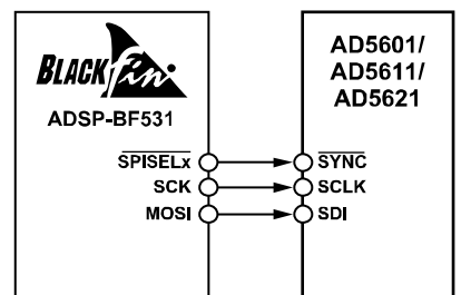
Figure 46. AD5601/AD5611/AD5621 to ADSP-BF531 Interface
