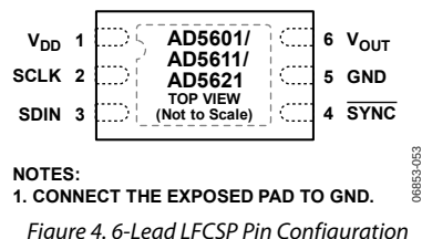
Figure 4. 6-Lead LFCSP Pin Configuration
