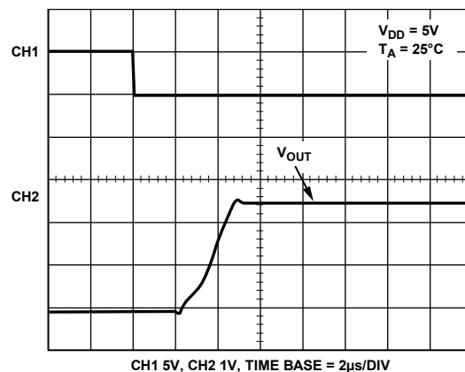
Figure 21. Exiting Power-Down Mode
