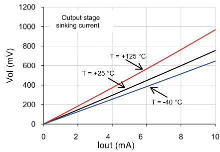
Figure 10: Output stage high-state saturation voltage vs. output current ( V_{sense} = 1\text{ V} )
