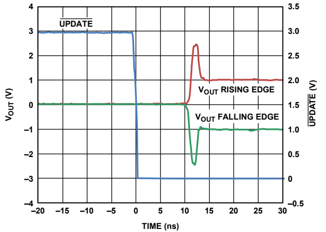
Figure 44. ADV3224 Enable Time
