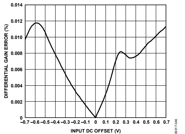
Figure 48. ADV3225 Differential Gain Error
