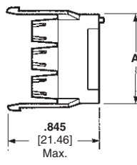
Cap Rear
