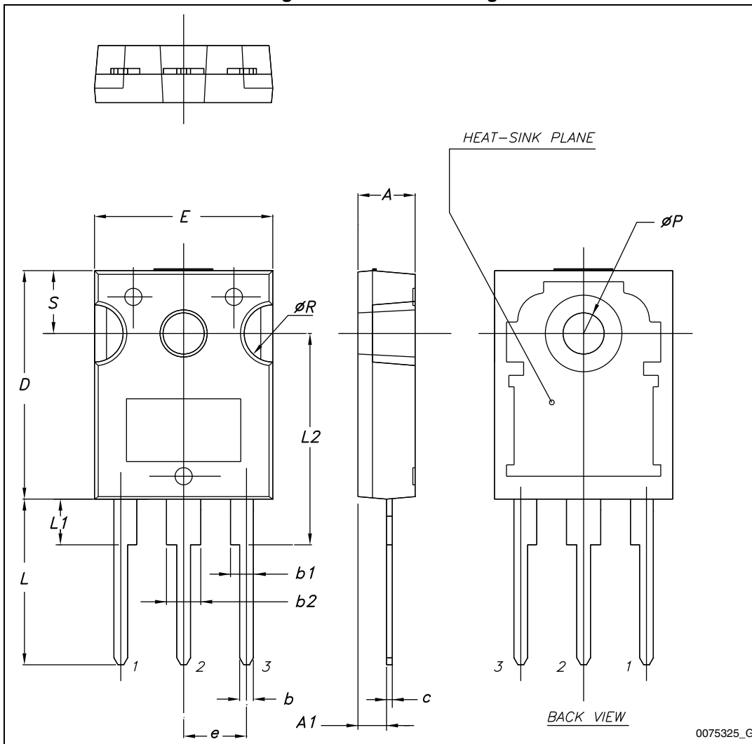
Figure 27. TO-247 drawing
