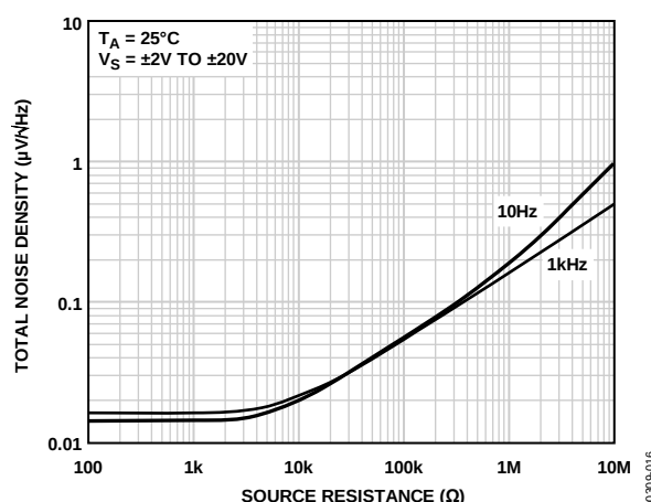
Figure 15. Total Noise Density vs. Source Resistance
