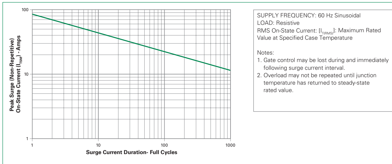
Figure 8: Surge Peak On-State Current vs. Number of Cycles
