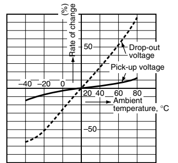
5.-(3) Change of pick-up and drop-out voltage (2a type) Sample: DSP2a-DC12V, 5 pcs.
