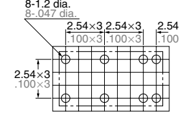
PC board pattern (Copper-side view) Single side stable 2 coil latching
