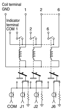
Fail-safe type
