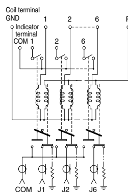
Latching type
