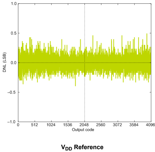
Figure 4.18. ADC Differential Linearity Error vs Code, V DD = 3 V, Temp = 25 °C
