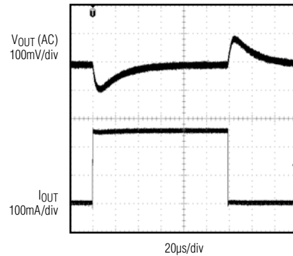
Figure 7. MAX17501F No Load to 250mA Load Transient
