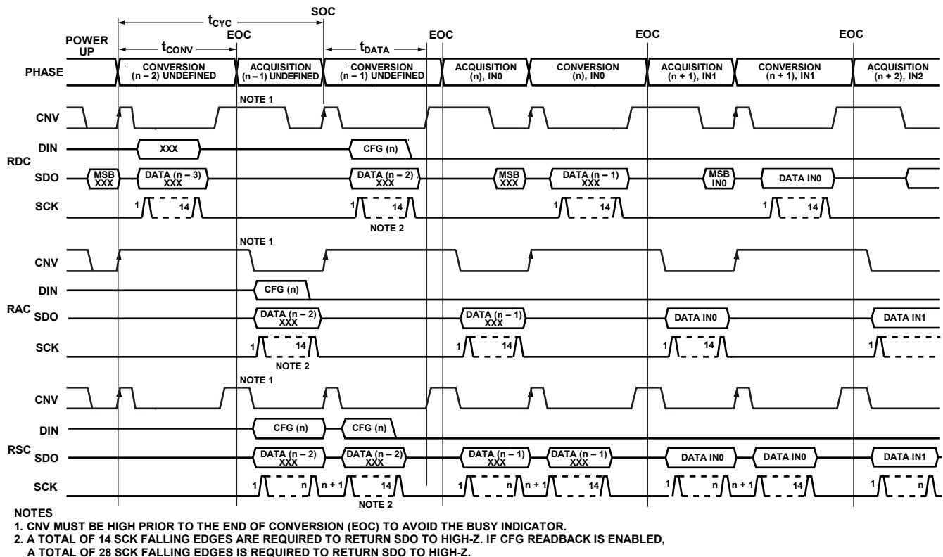
Figure 38. General Channel Sequencer Timing Without a Busy Indicator
