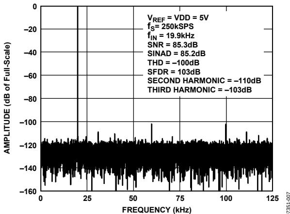
Figure 7. 20 kHz FFT, V_{REF} = V_{DD} = 5\text{ V}
