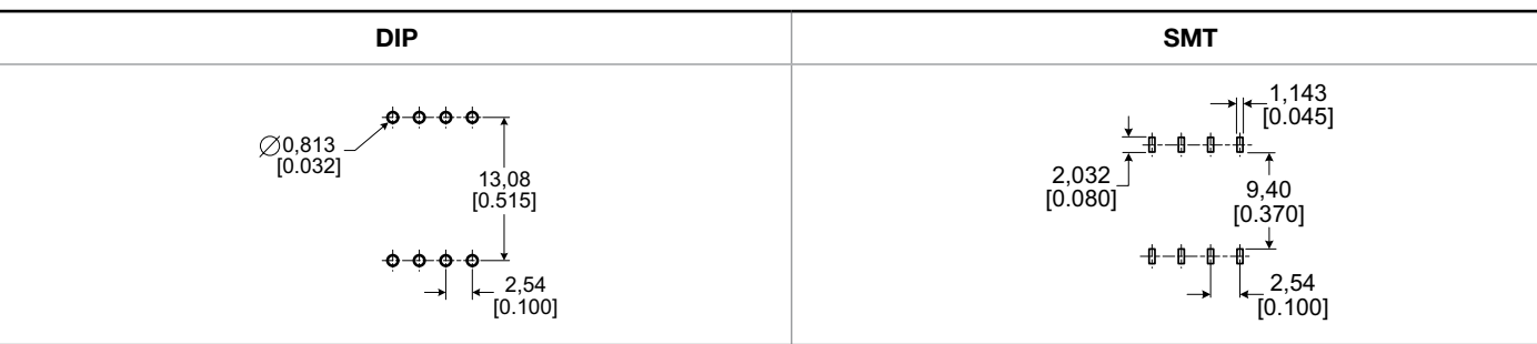
Figure 5. Recommended PCB Pad Layouts
