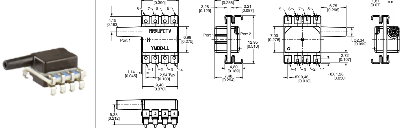
Figure 4. SMT Package Dimensional Drawings (continued)
