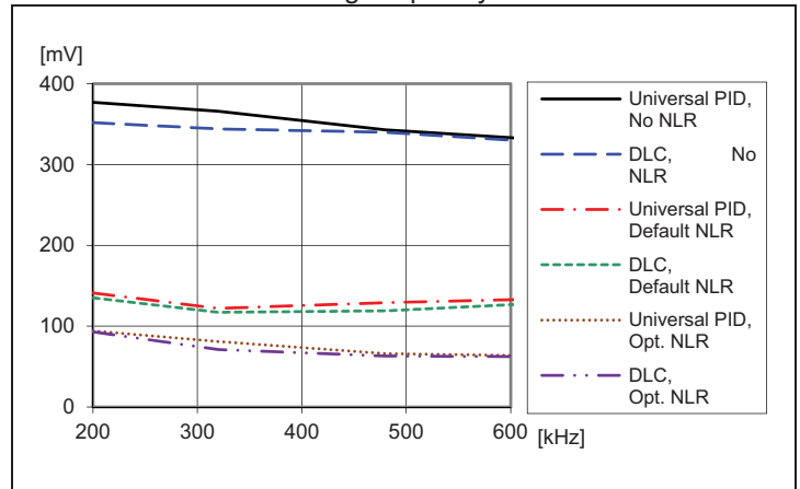
Load transient peak voltage deviation vs. frequency. Step-change (6.25-18.75-6.25 A). T_{P1} = +25\text{ }^\circ\text{C} , V_I = 12\text{ V} , V_O = 1.0\text{ V} , C_O = 470\text{ }\mu\text{F}/10\text{ m}\Omega
