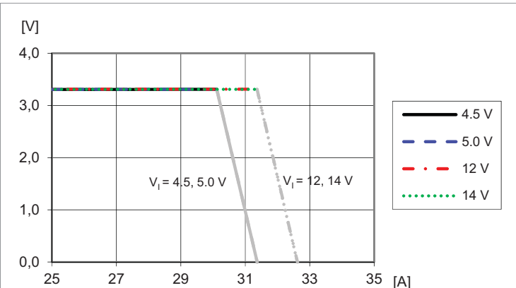
Output voltage vs. load current at T_{P1} = +25\text{ }^\circ\text{C} , V_O = 3.3\text{ V} . Note: Output enters hiccup mode at current limit.
