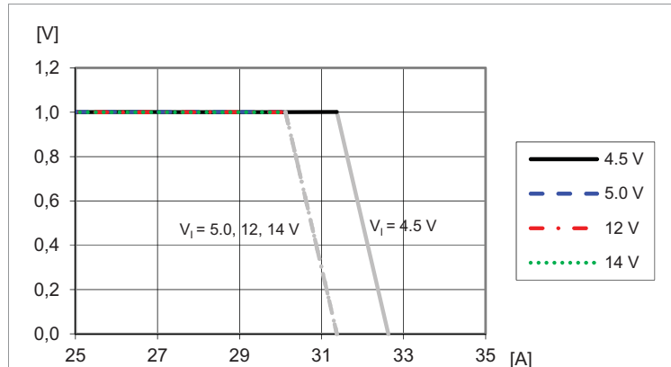
Output voltage vs. load current at T_{P1} = +25\text{ }^\circ\text{C} , V_O = 1.0\text{ V} . Note: Output enters hiccup mode at current limit.
