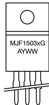
TO-220 FULLPACK CASE 221D STYLE 2
