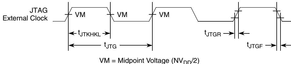
Figure 41. JTAG Clock Input Timing Diagram
