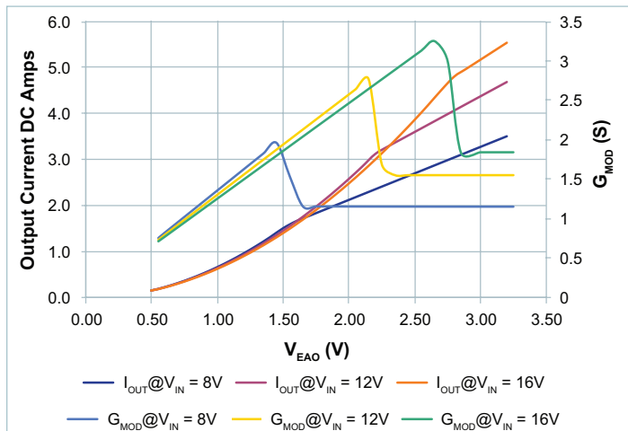
Figure 81 — G_{MOD} vs output current vs. V_{EAO} , V_{OUT} = 24V ; 8 – 16 V_{IN}
