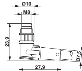
M8 x 1 male plug, angled version
