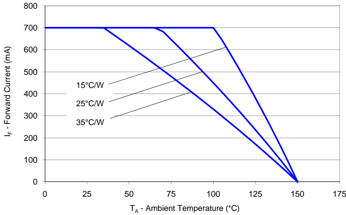
Figure 19. Maximum forward current vs. ambient temperature, based on T_{JMAX} = 150^{\circ}C , green LXML-PM01, cyan LXML-PE01, blue LXML-PB01 & royal-blue LXML-PR01 emitters..
