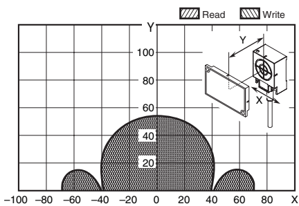
V680-HS65 (mounted on metallic material) & V680-D8KF68/-D32KF68 (Horizontal-facing RF Tag)
