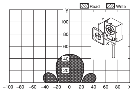
V680-HS63 (mounted on non-metallic material) & V680-D2KF67M (mounted on metallic surface: steel)
