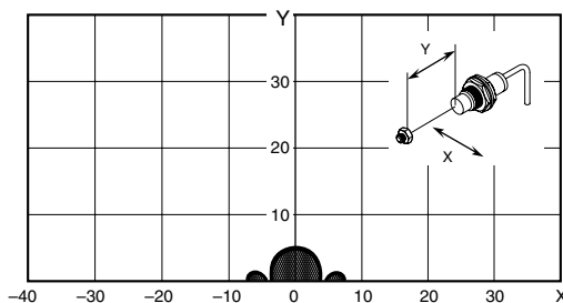
V680-D1KP52M-BT11 (mounted in metal/non-metallic material)
