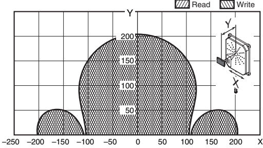
V680-H01-V2 (mounted on non-metallic material) & V680-D8KF68/-D32KF68 (Horizontal-facing RF Tag)
