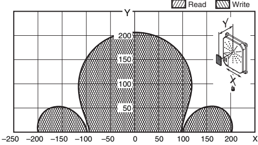
V680-H01-V2 (mounted on non-metallic material) & V680-D8KF68/-32KF68 (Vertical-facing RF Tag)
