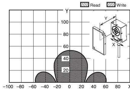
V680-HS65 (mounted on metallic material) & V680-D8KF68/-D32KF68 (mounted on non-metallic material) (Vertical-facing RF Tag)
