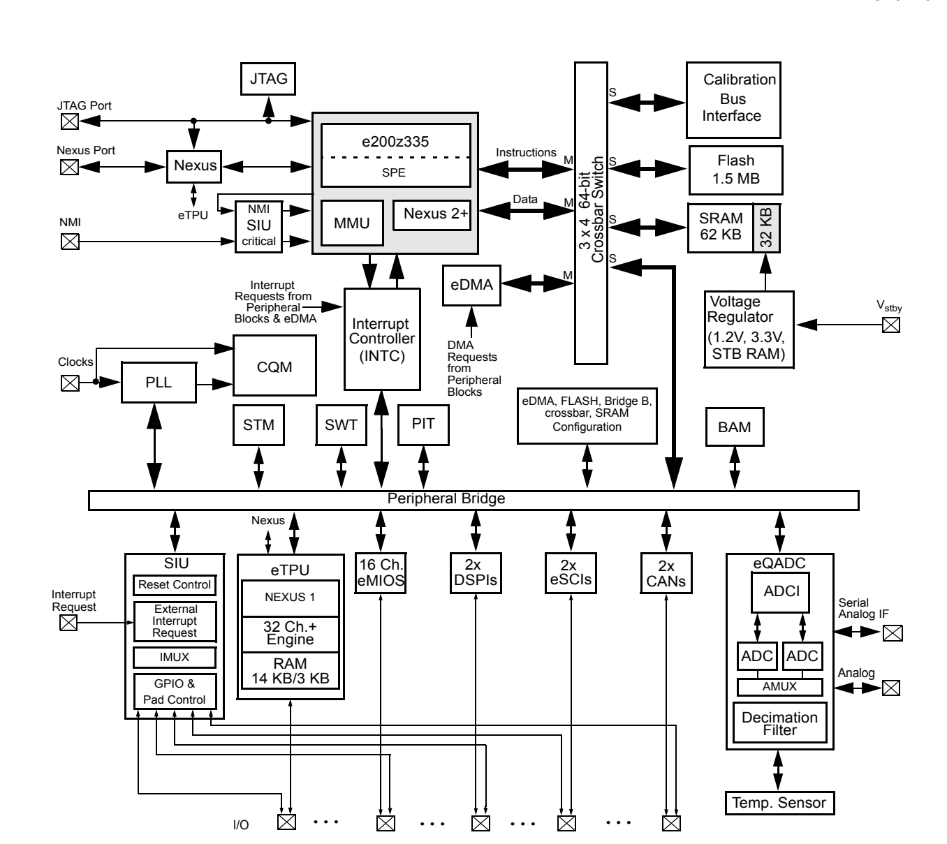
Figure 1. MPC5634M series block diagram
