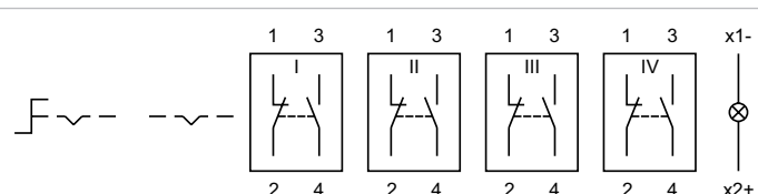
Wiring diagram 28
