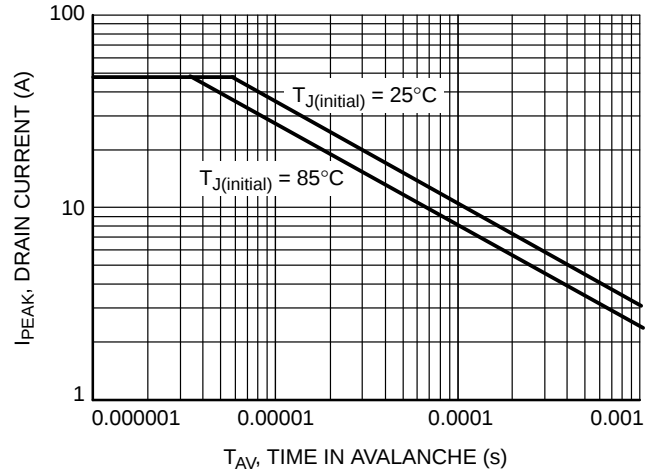
Figure 14. Avalanche Characteristics
