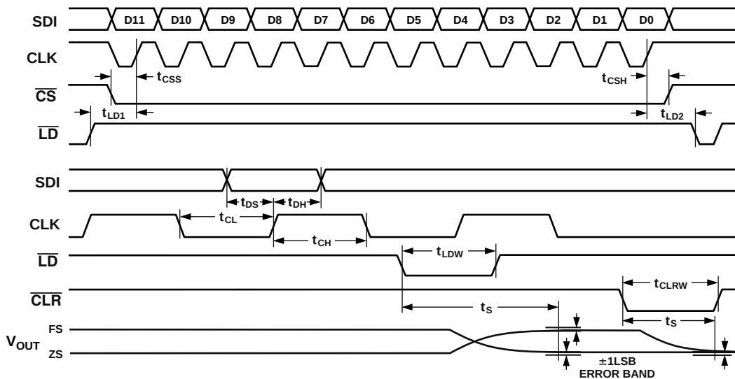
Figure 3. Timing Diagram
