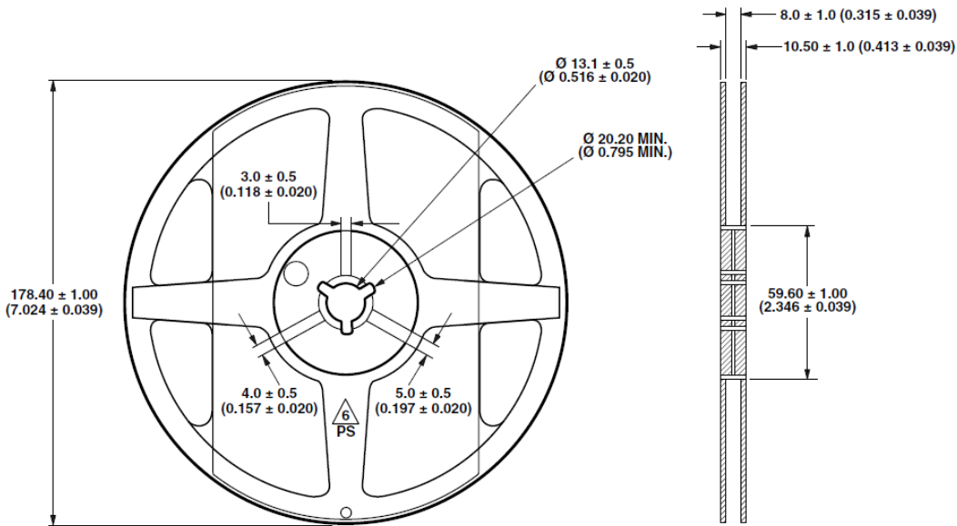
Figure 12: Reel Dimensions
