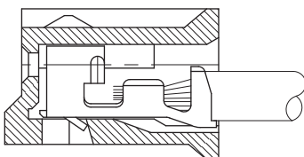
TERMINAL ASSEMBLY
