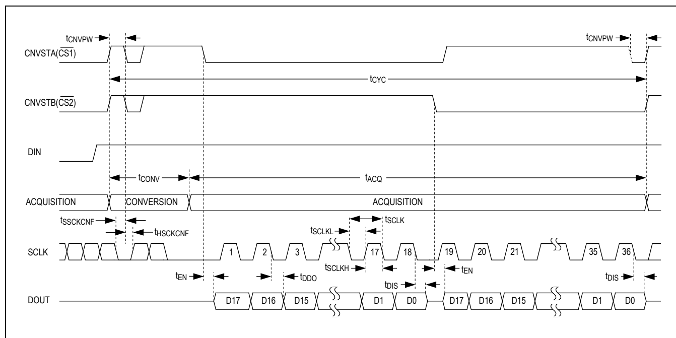
Figure 11. Multichannel \overline{\text{CS}} Configuration Timing
