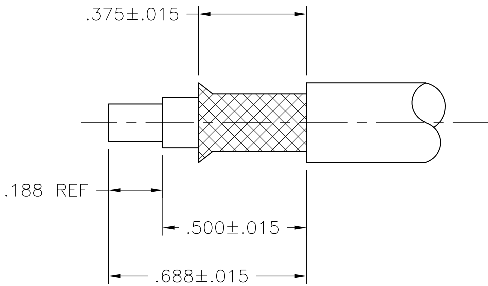
DETAIL X
