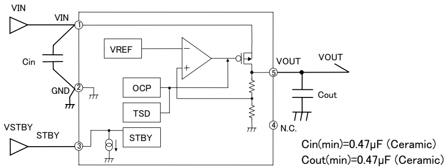
Figure 2. Block diagram
