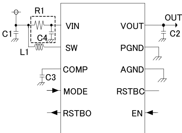
Figure 1. Application Circuit
