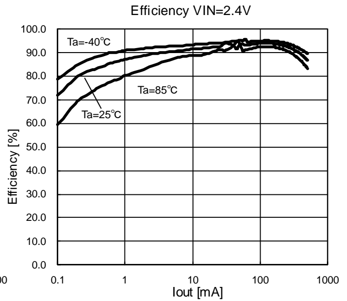
Figure 14. Efficiency PFM VIN=2.4V
