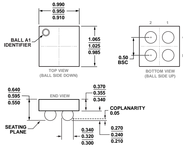
Figure 38. 4-Ball, Wafer Level Chip Scale Package [WLCSP] (CB-4-4) Dimensions show in millimeters
