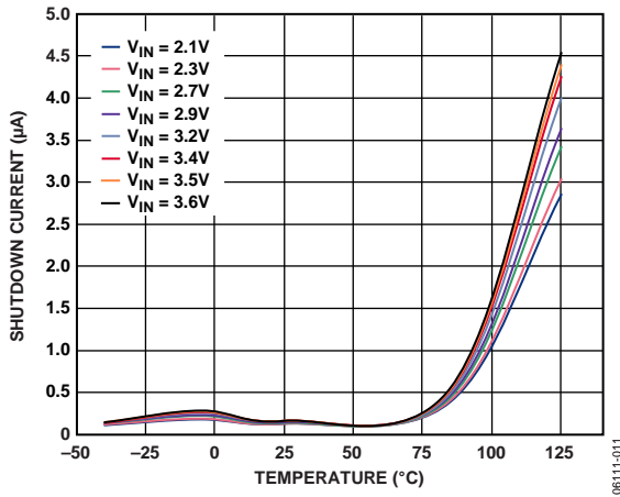
Figure 9. Shutdown Current vs. Temperature at Various Input Voltages
